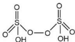
Peroxodisulphuric acid ( \text{H}_2\text{S}_2\text{O}_8 )
