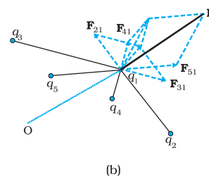
FIGURE 1.5 A system of (a) three charges (b) multiple charges.
