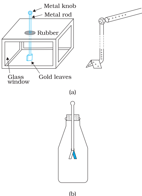
FIGURE 1.2 Electroscopes: (a) The gold leaf electroscope, (b) Schematic of a simple electroscope.
